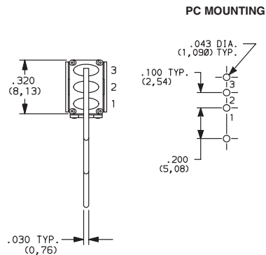
ET01SD1AV2BE Vertical Actuation SPDT
