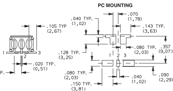
ET01M3D1SAPE Horizontal Actuation SPDT Only
