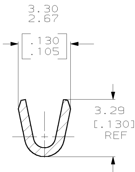
SECTION X-X
