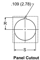
Panel Cutout
