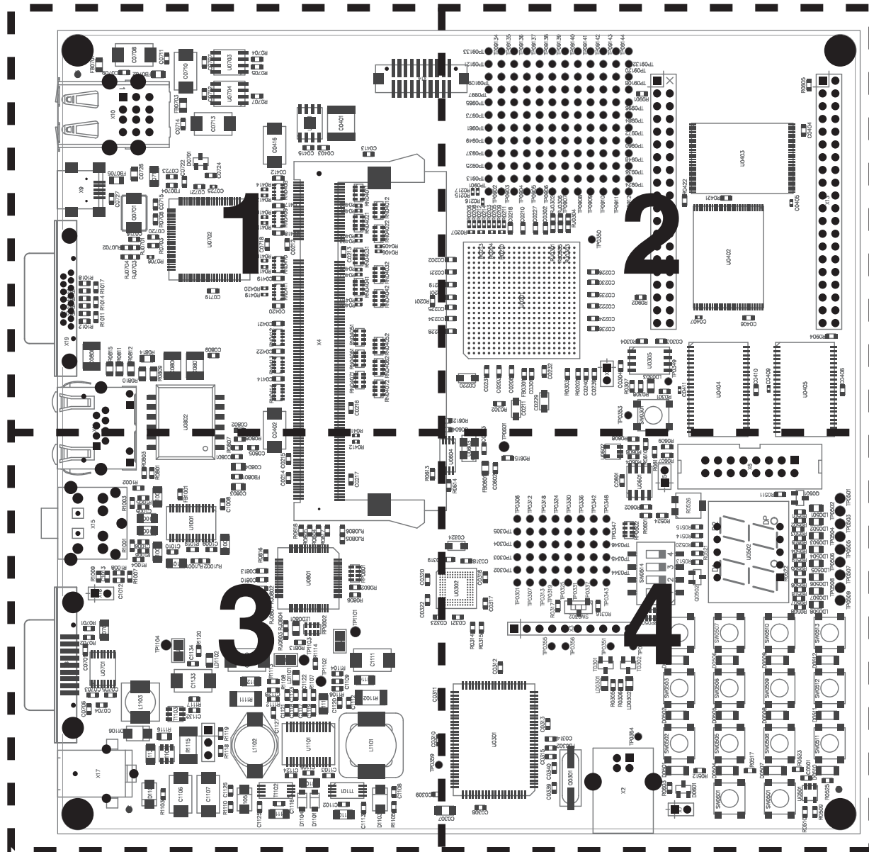
Figure 22. Assembly Diagram
