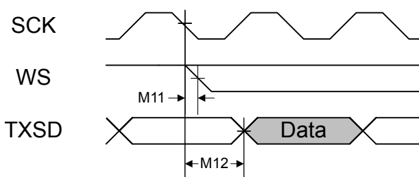
Figure 26-27. I 2 S Master Mode Transmit Timing
