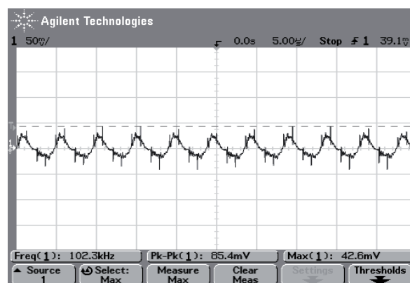
Figure 15 – Ripple Waveform ( V_{IN}=48V I_{OUT}=70A )
