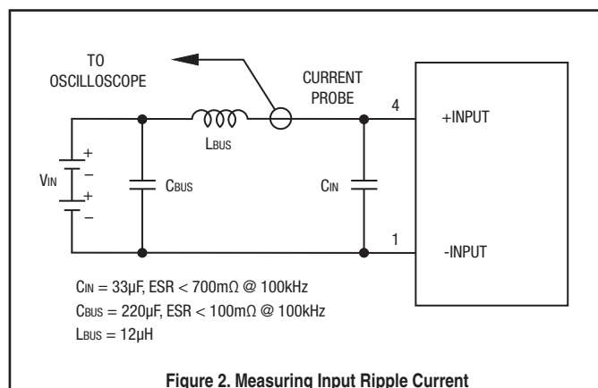
Figure 2. Measuring Input Ripple Current
