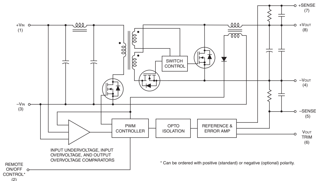
Figure 1. Simplified Schematic
