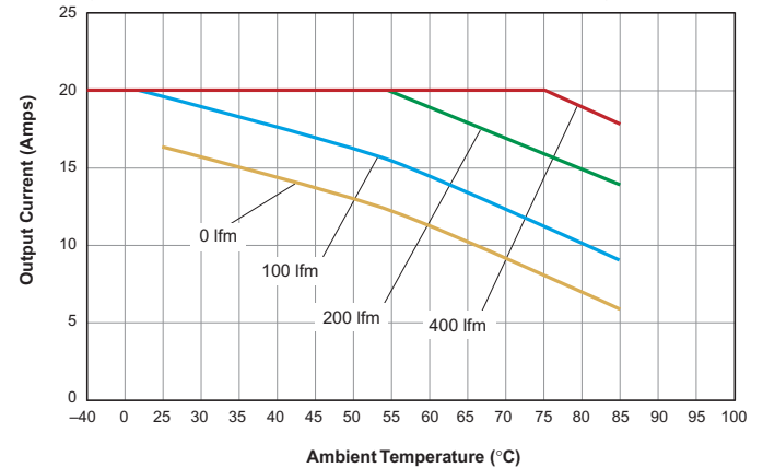
ULQ-3.3/20-D48
