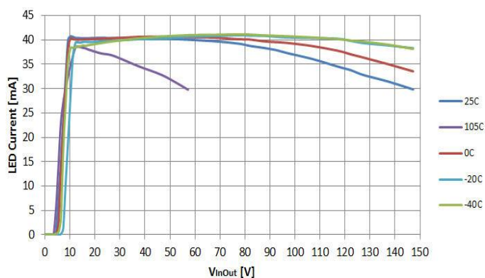
Figure 6. LED Current (-40°C to +105°C) vs. V_{IN\_OUT}
