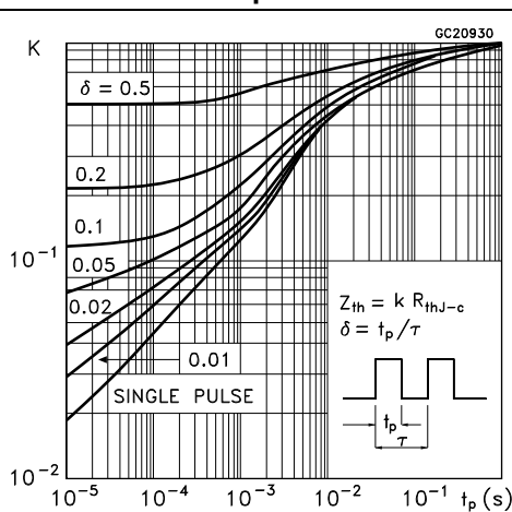
Figure 7. Thermal impedance TO-247
