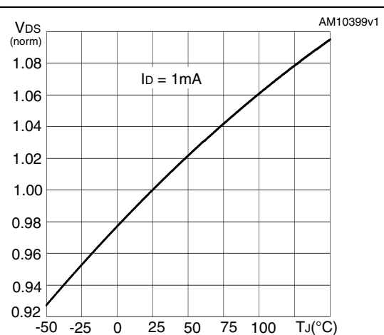
Figure 17. Normalized B_{VDS} vs temperature
