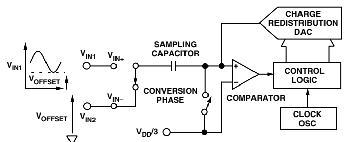
Figure 6. Pseudo Differential Input Scheme
