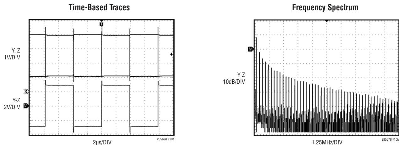
Figure 10. LTC2858-1 Driver Output at 100kHz Into 100 \Omega Resistor
