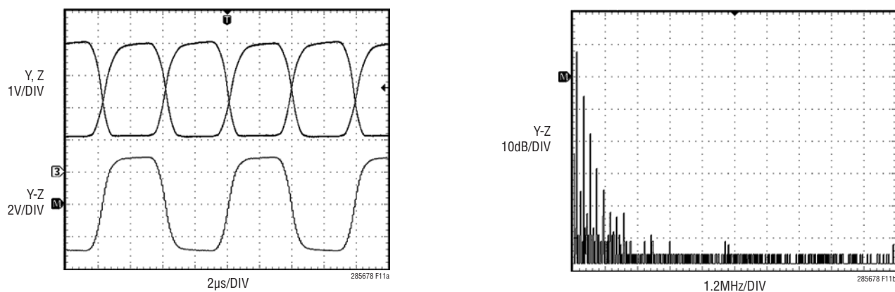
Figure 11. LTC2858-2 Driver Output at 100kHz Into 100 \Omega Resistor
