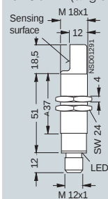
3RG62 2. (angled sensor)
