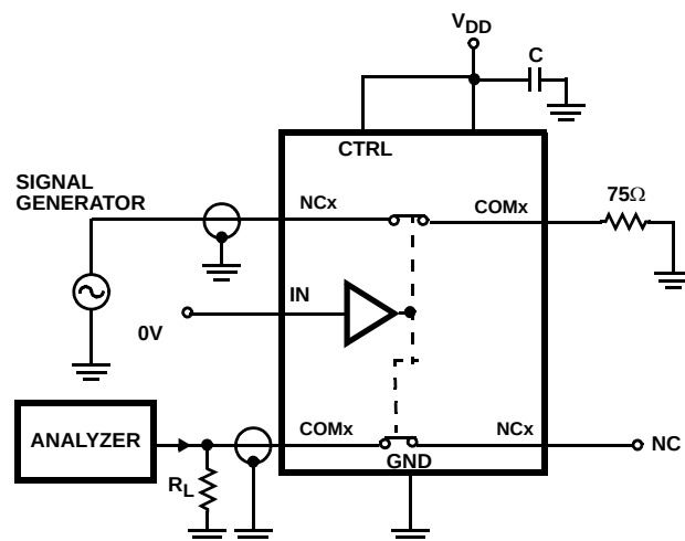
FIGURE 6. NCx CROSSTALK TEST CIRCUIT
