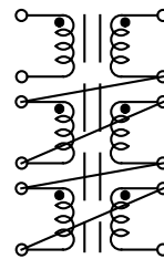
Figure 3 Turns ratio: 1:5 or 5:1
