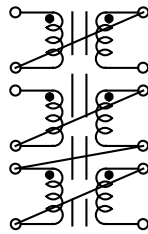
Figure 6 Turns ratio: 1:2 or 2:1
