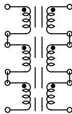
Figure 2 Turns ratio: 1:1
