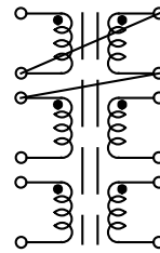
Figure 8 Turns ratio: 3:1:1:1
