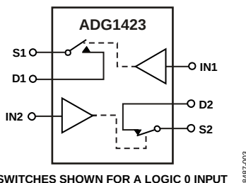
Figure 3. ADG1423 Functional Block Diagram
