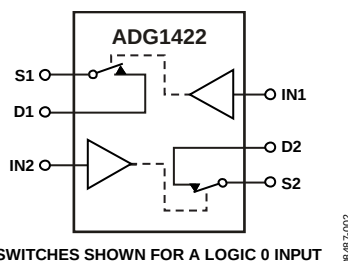
Figure 2. ADG1422 Functional Block Diagram
