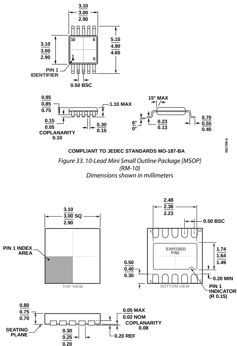
Figure 34. 10-Lead Lead Frame Chip Scale Package [LFCSP_WD] 3 mm x 3 mm Body, Very Thin, Dual Lead (CP-10-9) Dimensions shown in millimeters
