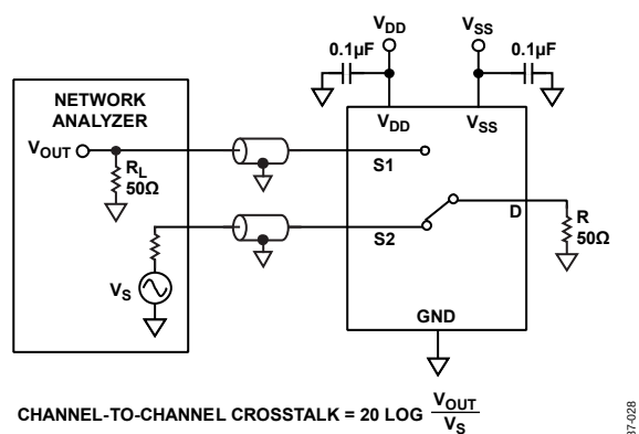
Figure 30. Channel-to-Channel Crosstalk
