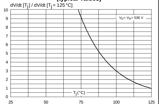
Figure 13: Relative variation of static dV/dt immunity versus junction temperature (typical values)
