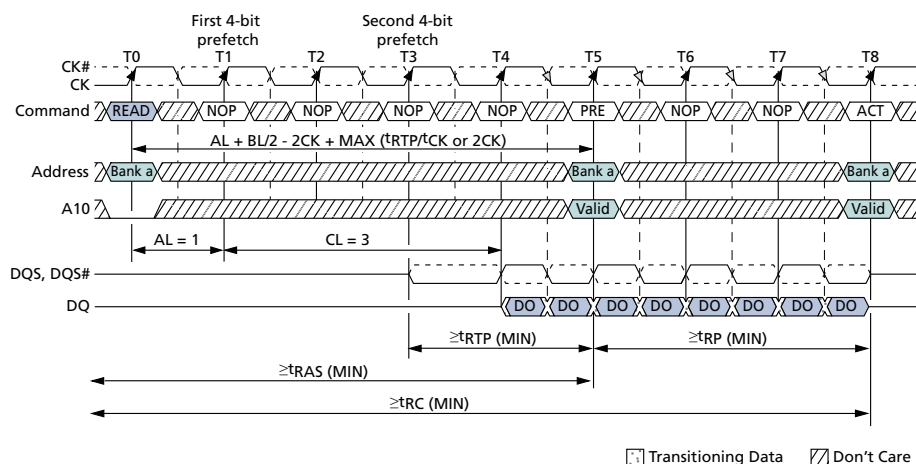
Figure 51: READ-to-PRECHARGE – BL = 8
