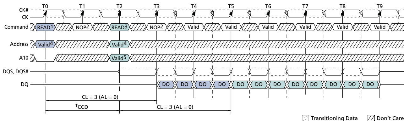
Figure 48: READ Interrupted by READ
