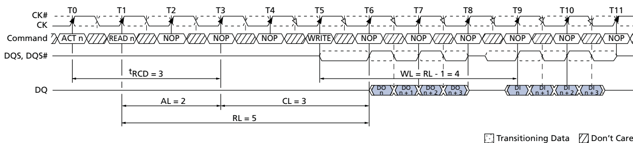
Figure 49: READ-to-WRITE
