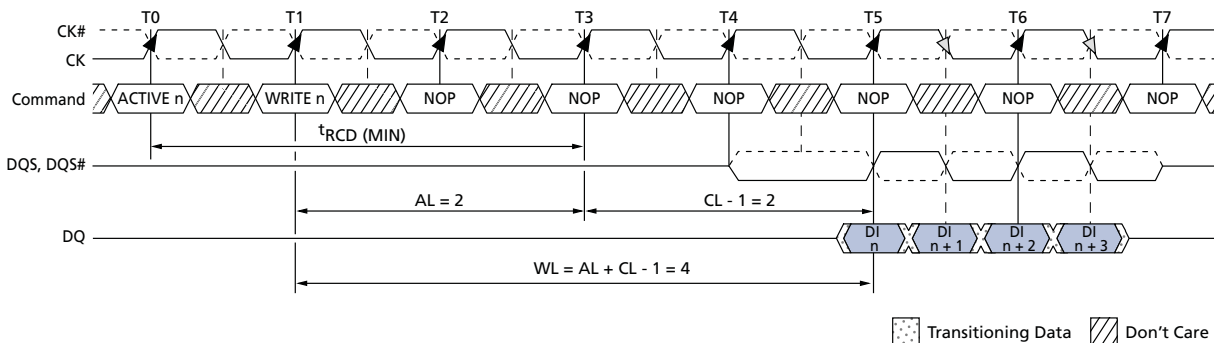
Figure 39: WRITE Latency
