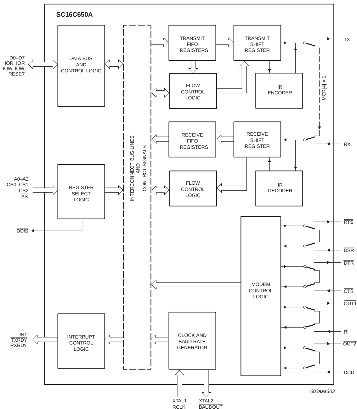
Fig 7. Internal loop-back mode diagram.
