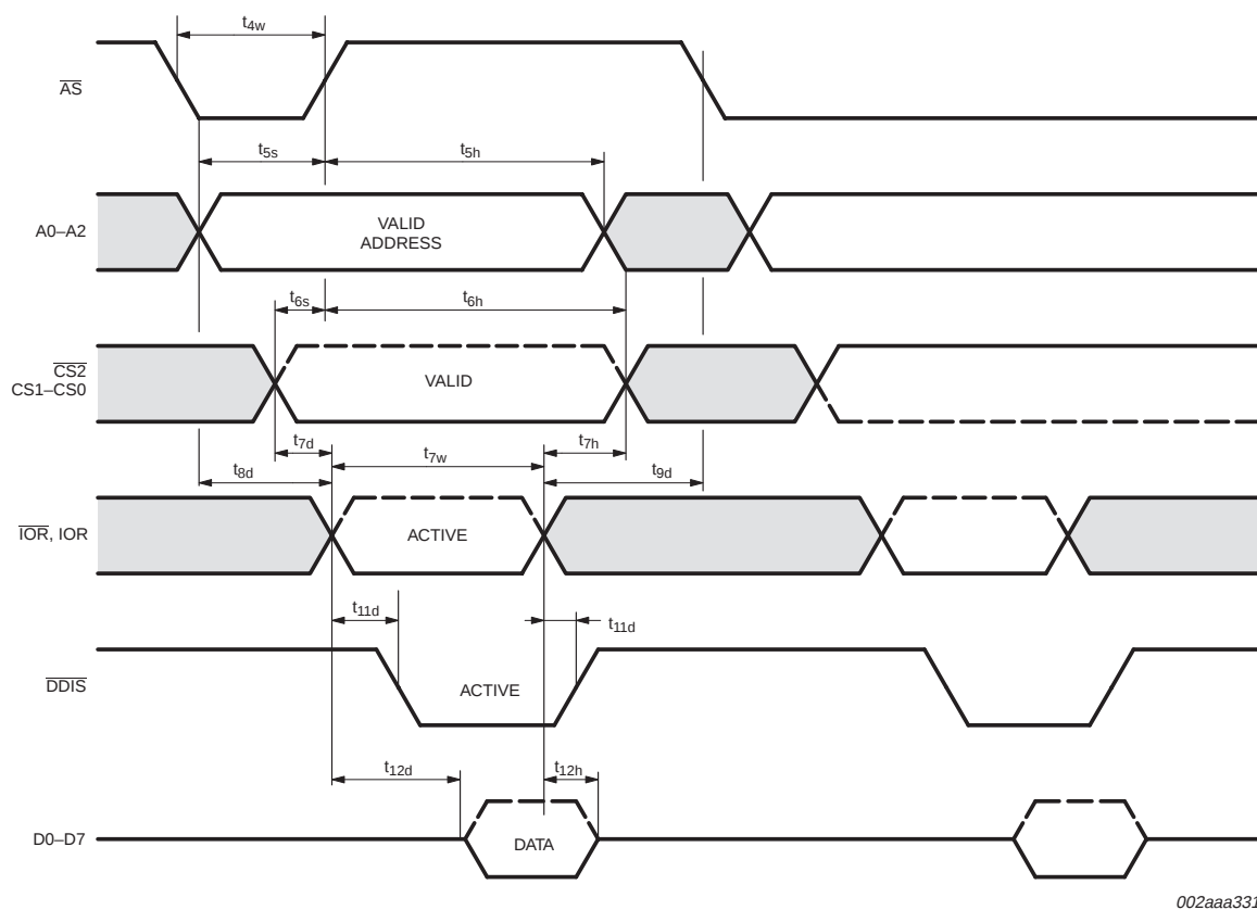
Fig 8. General read timing when using \overline{\text{AS}} signal.
