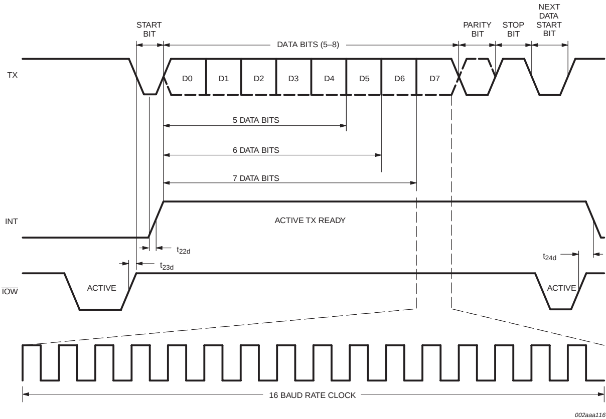
Fig 17. Transmit timing.
