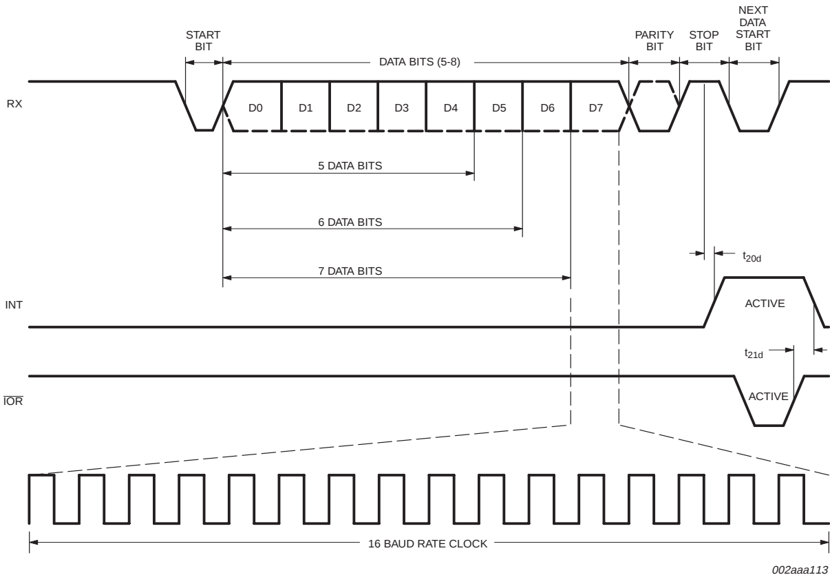
Fig 14. Receive timing.
