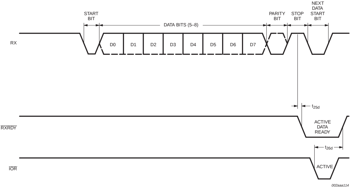
Fig 15. Receive ready timing in non-FIFO mode.
