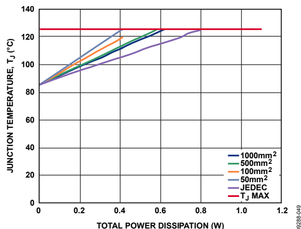
Figure 60. Junction Temperature vs. Total Power Dissipation, T_A = 85^\circ\text{C}
