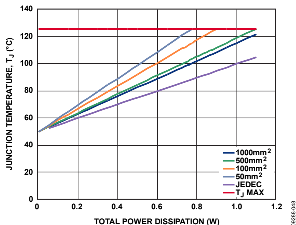
Figure 59. Junction Temperature vs. Total Power Dissipation, T_A = 50^\circ\text{C}
