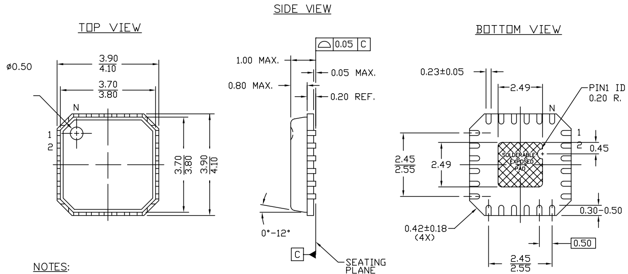
Figure 6. 24-pin QFN (4 × 4 mm) 2.49 × 2.49 E-Pad (Subcon Punch Type Package) Package Outline, 51-85203
