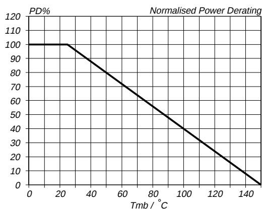
Fig.4. Normalised limiting power dissipation. P_D\% = 100 \cdot P_D / P_D(25^\circ\text{C}) = f(T_{mb})
