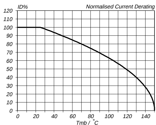
Fig.5. Normalised continuous drain current. I_D\% = 100 \cdot I_D / I_D(25^\circ\text{C}) = f(T_{mb}) ; conditions: V_{IS} = 5\text{ V}
