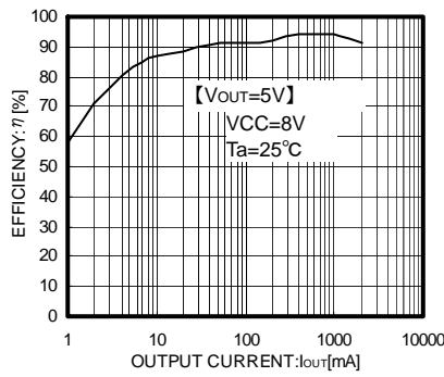
Fig.7 Efficiency
