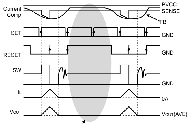
Fig.23 SLLM TM Not switching timing chart
