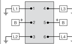
DPDT On-On (6 terminals) Diagram D
