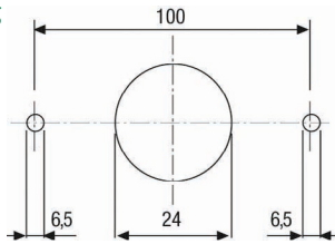
Mounting Diagram
