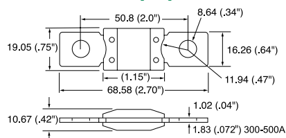
Dimensions inches [mm]
