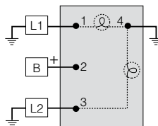
SPDT On-Off-On or On-On with Dependent & Independent Lights (Four terminals) Diagram J
