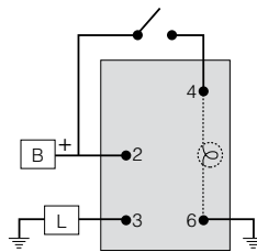
SPST Off-Off - Independent Illumination (Four terminals) Diagram G1
