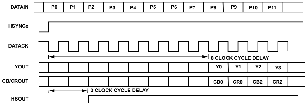
Figure 15. 4:2:2 Timing Mode
