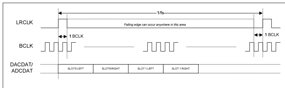
Figure 62 TDM in DSP Mode B
