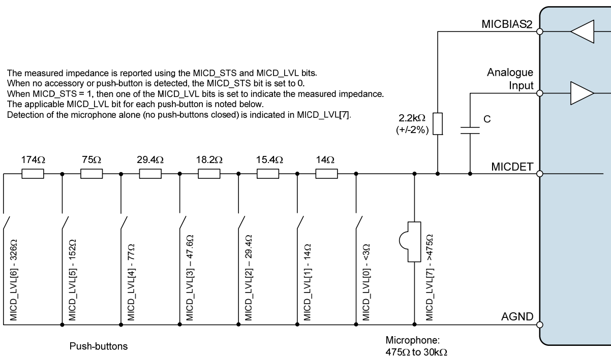
Figure 88 External Accessory Detect Connection
