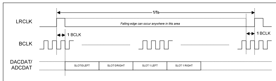
Figure 61 TDM in DSP Mode A
