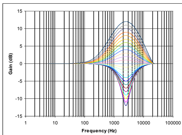
Figure 27 EQ Band 4 – Peak Filter Response
