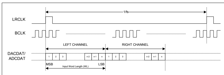
Figure 55 DSP B Mode ( AIFnDAC\_LRCLK\_INV / AIFnADC\_LRCLK\_INV=1 , Master)
