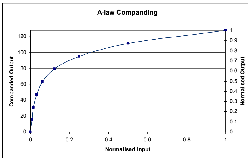
Figure 65 A-Law Companding
