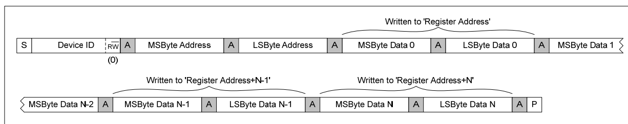
Figure 77 Multiple Register Write to Specified Address using Auto-increment
