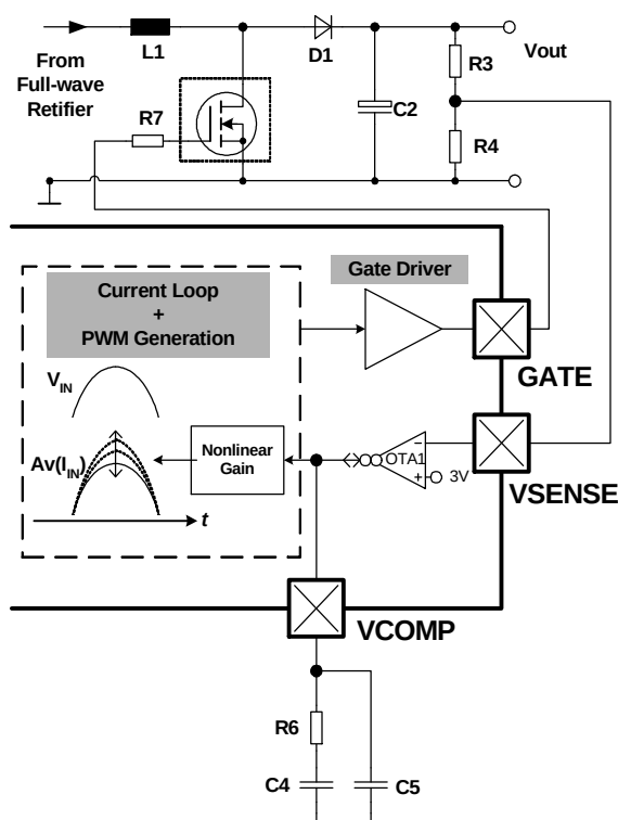
Figure 15 Voltage Loop
