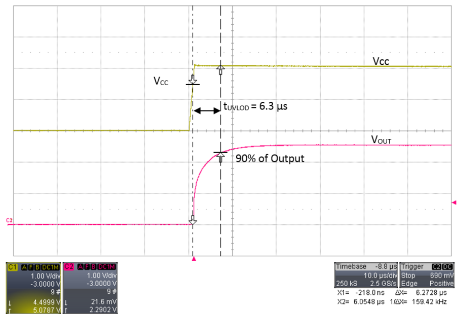
UVLO Enable Time ( t_{UVLOD} ) I_P = 0\text{ A} , C_{BYPASS} = \text{Open} , C_L = \text{Open} V_{CC} 3 V to 5 V recovery time = 1 \mu\text{s}
