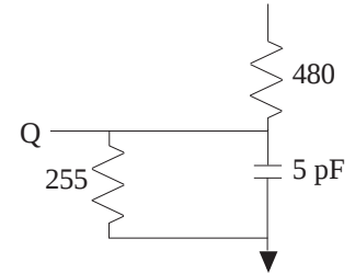
Fig. 2 Output Load Equivalent
