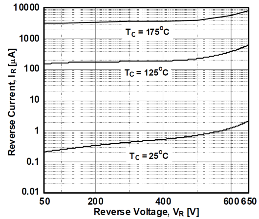
Figure 20. Reverse Current
