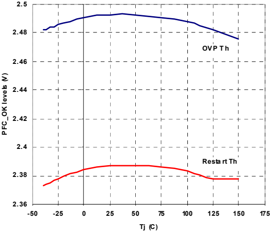
Figure 11. OVP levels vs. T_J
