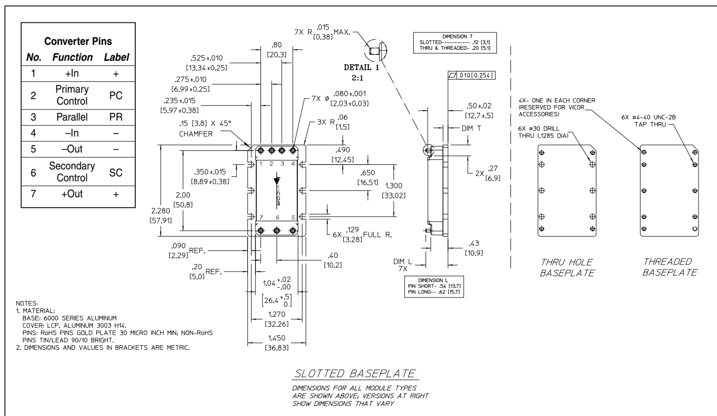
Figure 13 — Module outline
