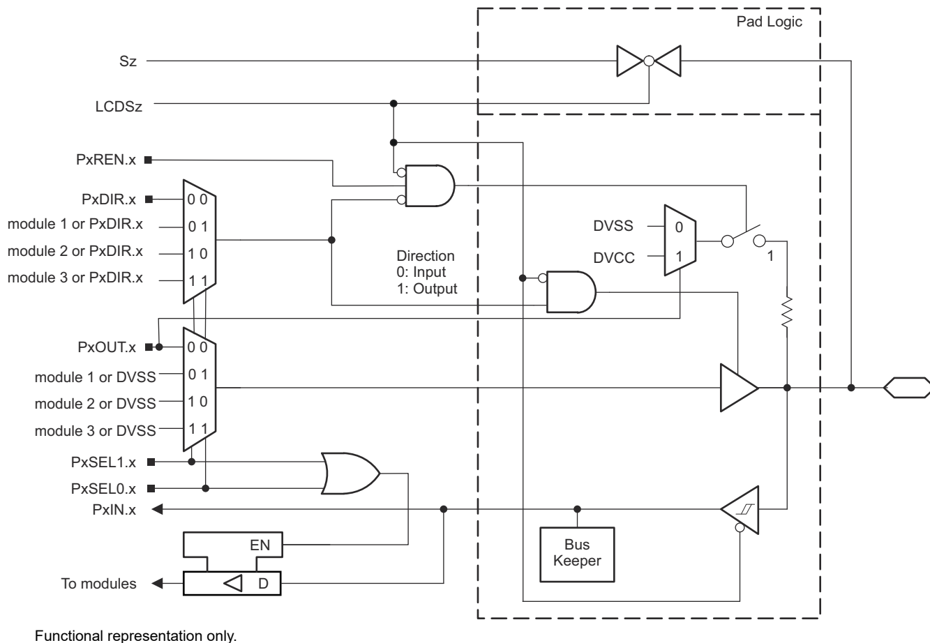
Figure 9-7. Port P3 (P3.0 to P3.7) Diagram
