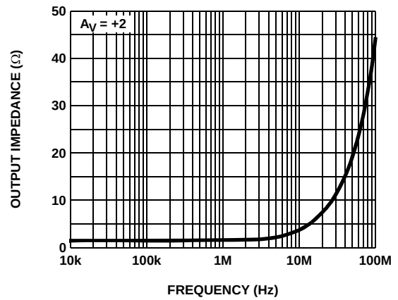
FIGURE 20. OUTPUT IMPEDANCE
