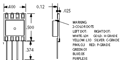
No Pressure Port
