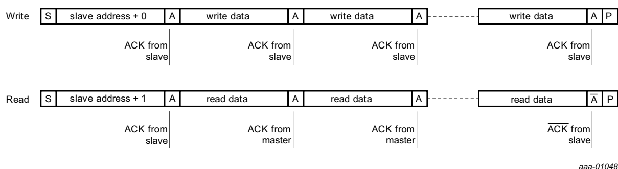
Fig 17. I 2 C read and write protocol
