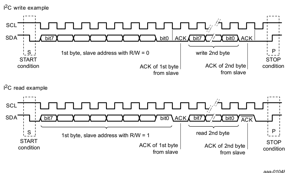
Fig 18. I 2 C read and write signaling
