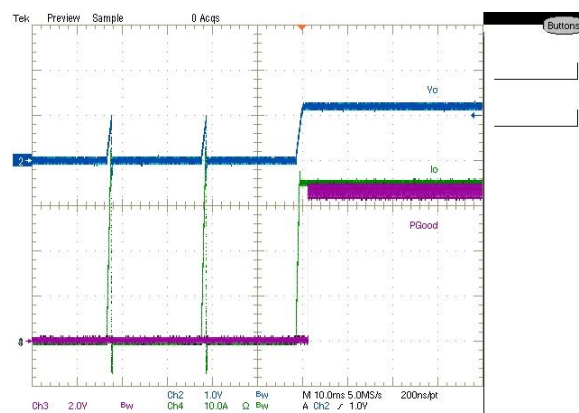
Figure 43: Recovery from Hiccup CH2:Vout, CH3:PGood, CH4:Iout
