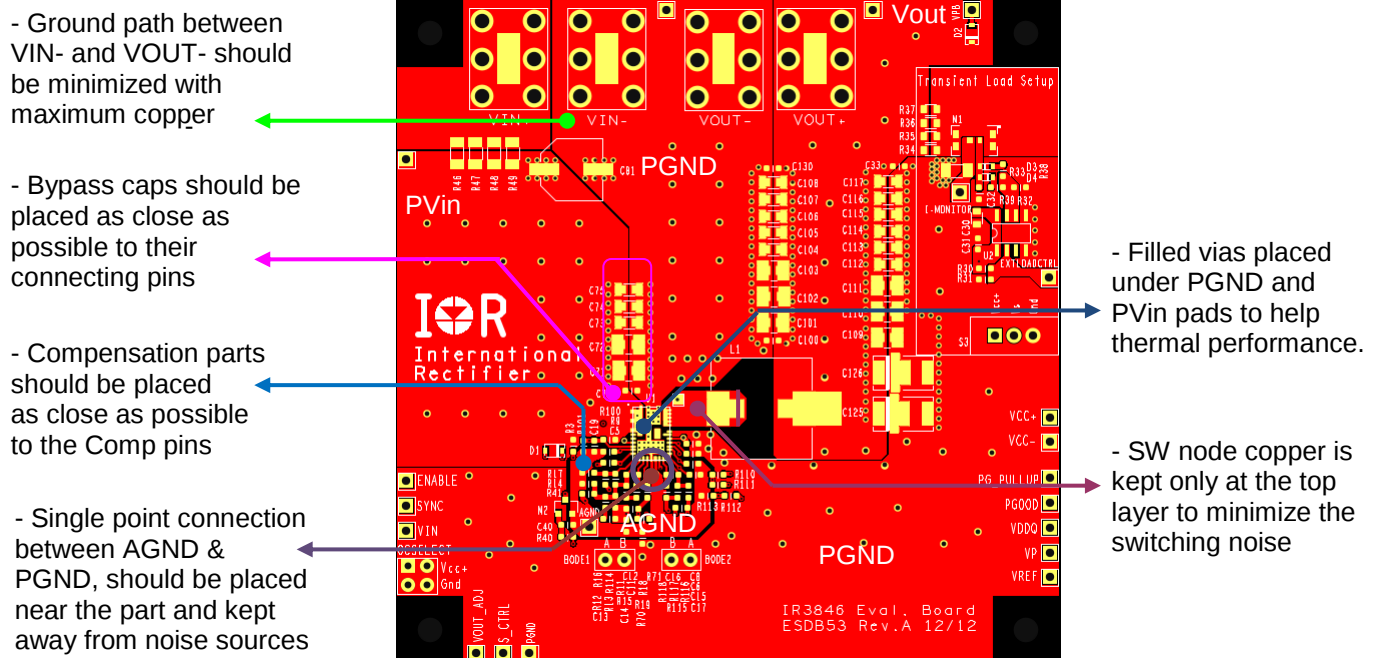
Figure 51a: IRDC3846 Demo board Layout Considerations – Top Layer
