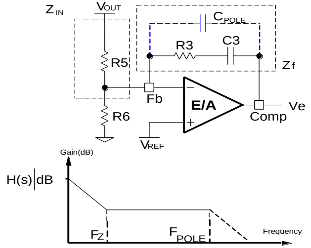
Figure 35: Type II compensation network and its asymptotic gain plot
