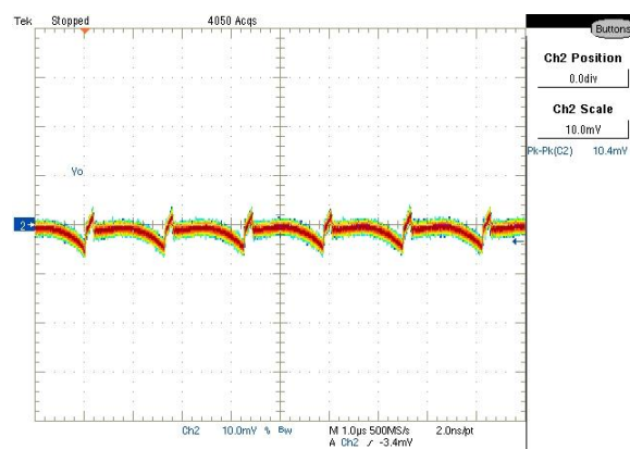
Figure 45: Output Voltage Ripple at full load CH2:Vout
