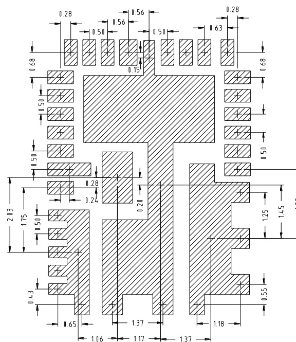
PAD SPACING
