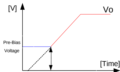
Figure 8: Pre-Bias startup
