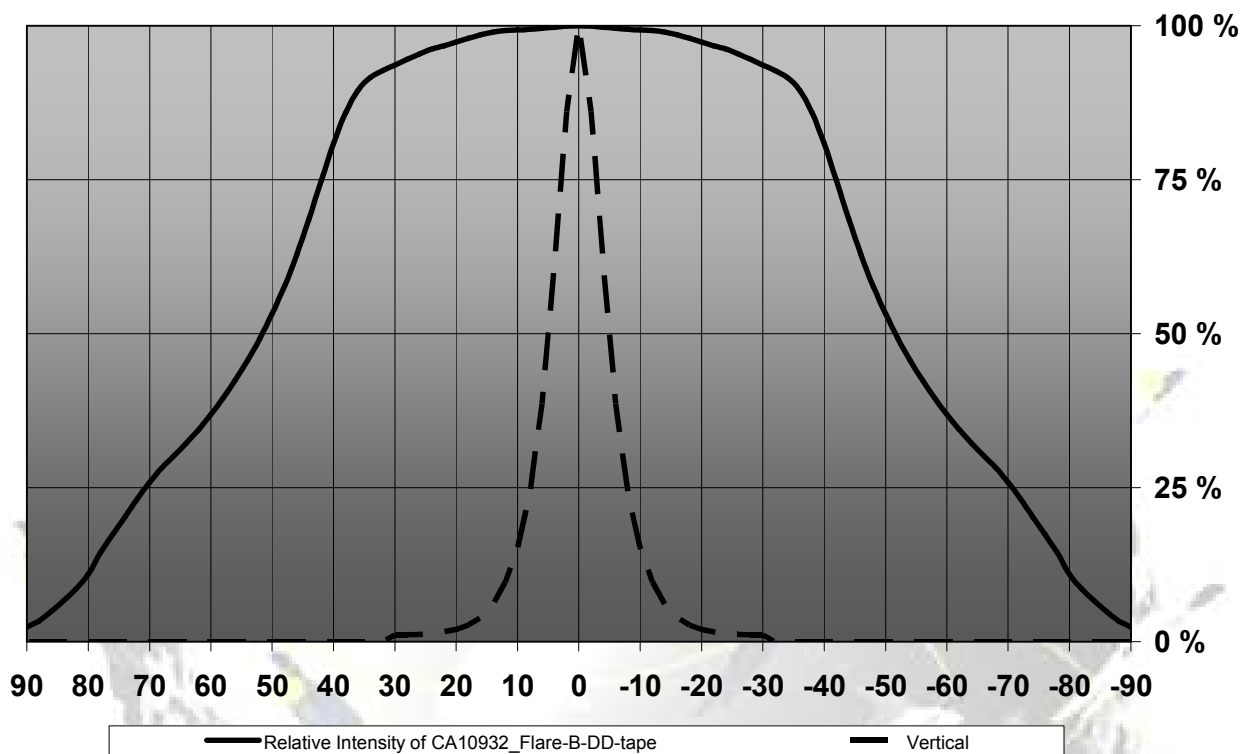
Relative Intensity of CA10932_Flare-B-DD-tape
