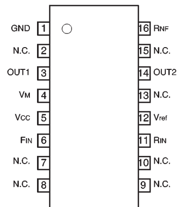
Fig.1 Pin assignments
