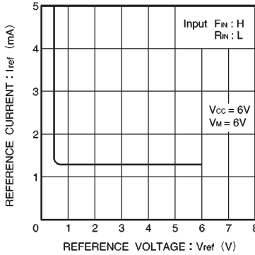
Fig.11 V_{REF} reference current vs. V_{REF} reference voltage
