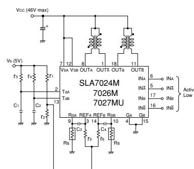
Active Low
