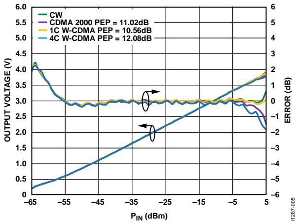
Figure 5. Error from CW Linear Reference vs. Signal Modulation (CDMA 2000, One-Carrier W-CDMA, Four-Carrier W-CDMA), Frequency = 2.14 GHz, C RMS = 0.1 μF, Three Point Calibration at 0 dBm, -40 dBm, and -55 dBm
