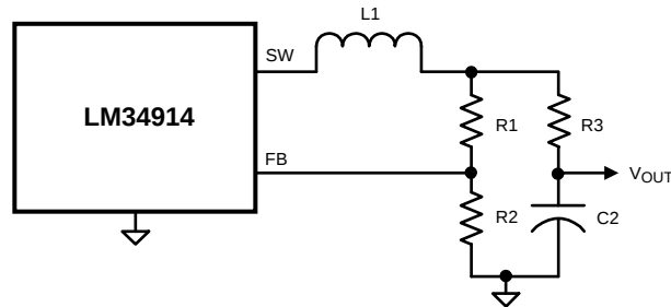
Figure 13. Alternate Minimum Output Ripple
