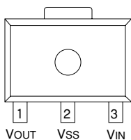
SOT-89 (TOP VIEW)
