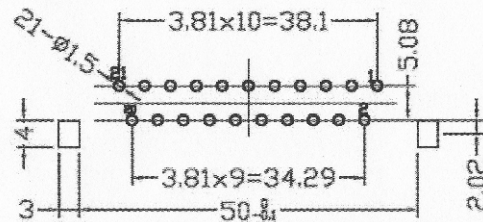
PCB HOLE PATTERN
