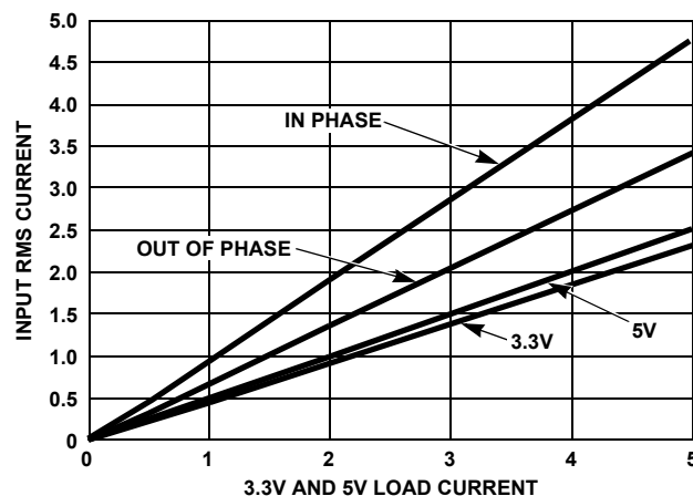
FIGURE 19. INPUT RMS CURRENT vs LOAD
