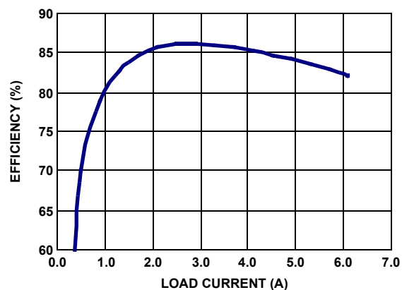
FIGURE 5. PWM2 EFFICIENCY vs LOAD ( V_{\text{O}} = 1.5\text{V} ), V_{\text{IN}} = 12\text{V} , 1 DUAL SO-8 MOSFET (IRF7907) FOR UPPER AND LOWER MOSFETS
