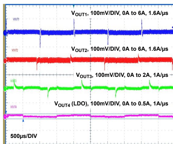
FIGURE 13. OUTPUT RIPPLE UNDER TRANSIENT LOAD
