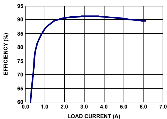
FIGURE 3. PWM1 EFFICIENCY vs LOAD ( V_{\text{O}} = 2.5\text{V} ), V_{\text{IN}} = 12\text{V} , 1 DUAL SO-8 MOSFET (IRF7907) FOR UPPER AND LOWER MOSFETS
