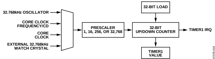
Figure 24. Timer1 Block Diagram
