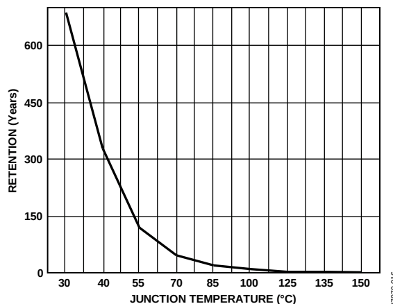
Figure 22. Flash/EE Memory Data Retention
