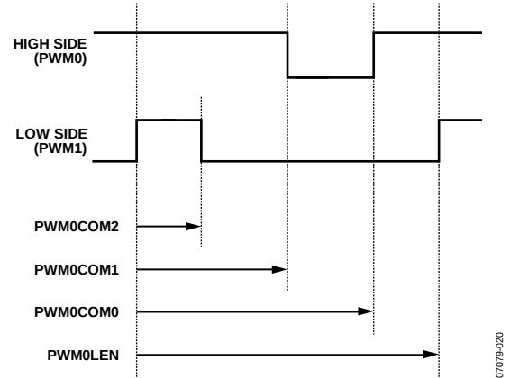
Figure 26. PWM Timing
