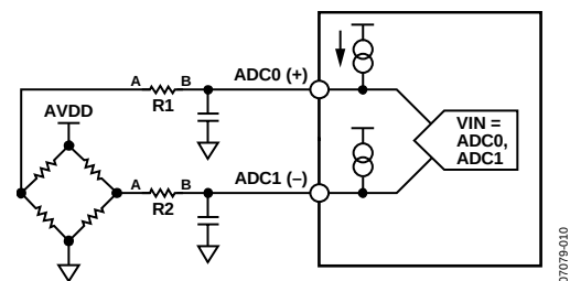
Figure 15. Example Circuit Using Diagnostic Current Sources
