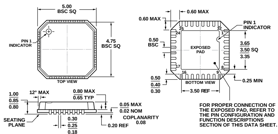
Figure 30. 32-Lead Lead Frame Chip Scale Package [LFCSP_VQ] 5 mm x 5 mm Body, Very Thin Quad (CP-32-4) Dimensions shown in millimeters
