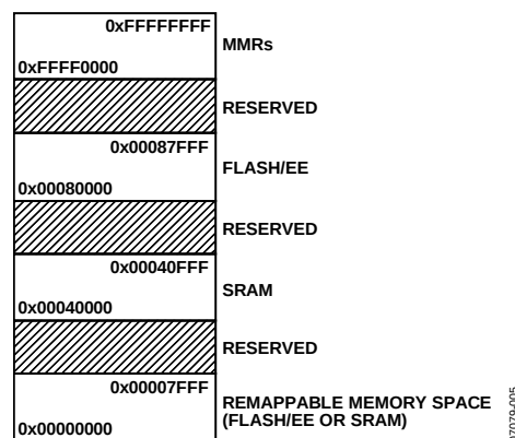
Figure 10. Memory Map
