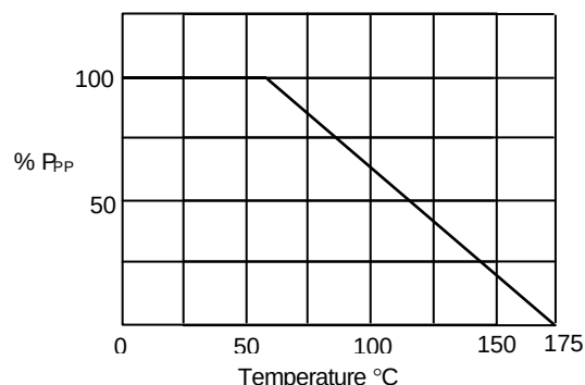
Figure 4 - Derating Curve
