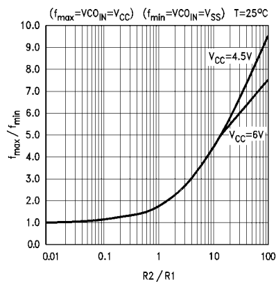
Typical f_{max}/f_{min} vs R2/R1
