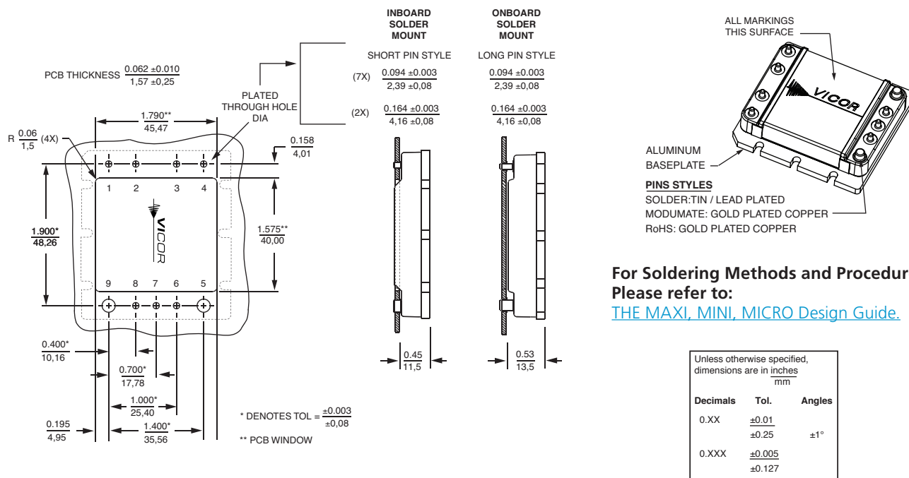
Figure 13 — PCB mounting specifications
