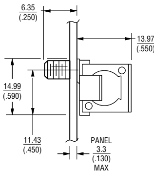
PANEL LAYOUT
