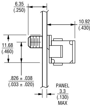
PANEL LAYOUT
