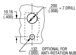
PANEL LAYOUT
