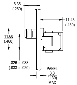
PANEL LAYOUT
