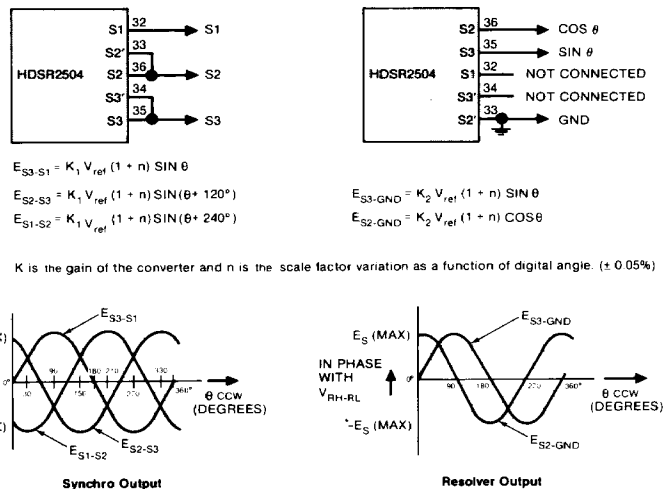
FIGURE 7 Synchro/Resolver Outputs
